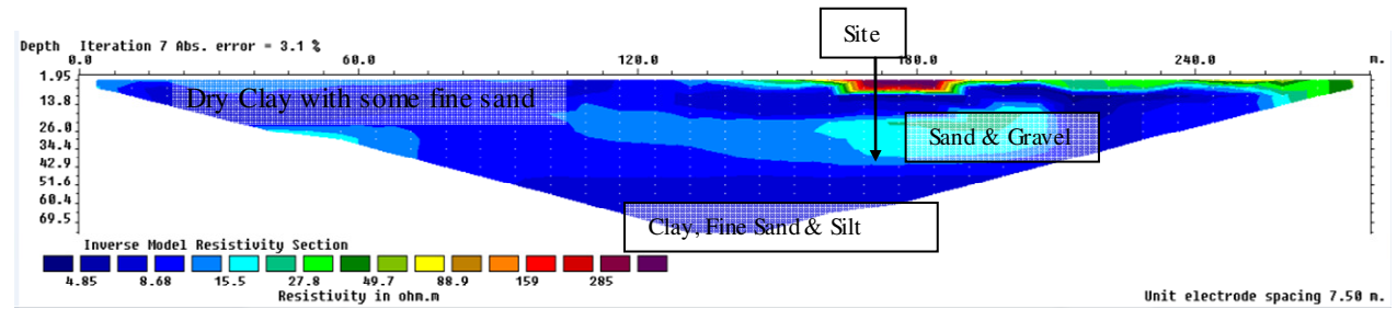
LP No 1 Half Schlumberger
