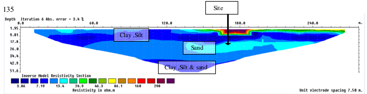
LP No 1 Schlumberger Electrode Configuration.
